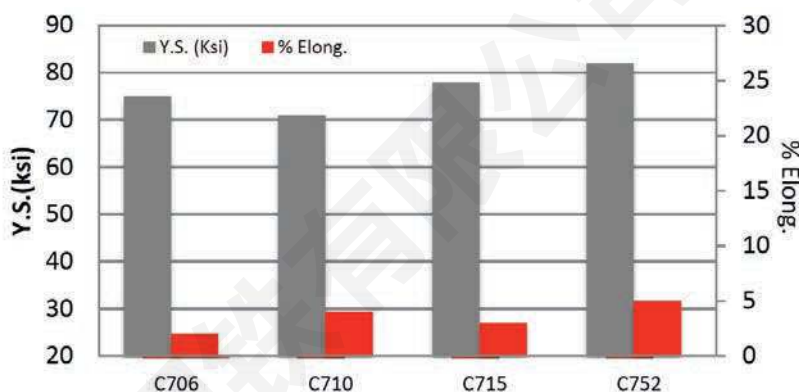
Figure 1: Comparison of Yield Strength and Elongation performance of select Hard temper Cupro-Nickel materials.
