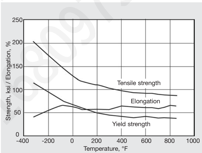
Figure 2. Effect of temperature on mechanical properties of annealed INCOLOY alloy 27-7MO
