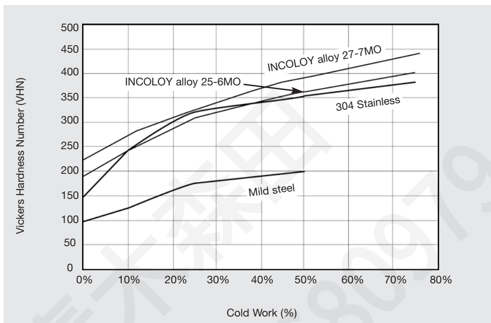
Figure 7. Effect of cold work on hardness.
