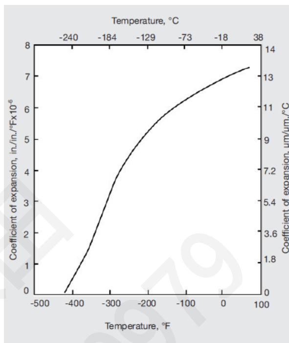
Figure 1 – Thermal Expansion at Low Temperatures
