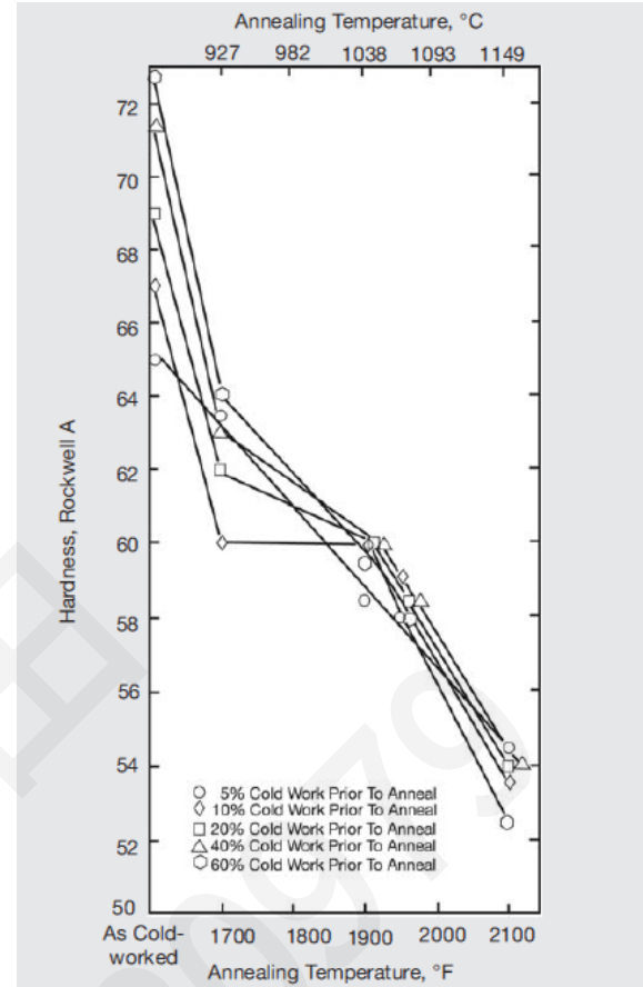
Figure 8 – Effect of annealing temperature on the hardness Of sheet (30 min at temperature).
