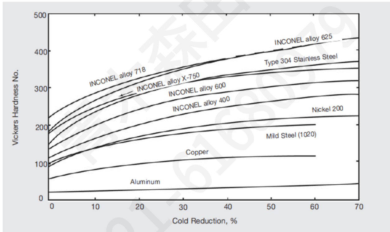
Figure 18 – Effect of cold work on hardness.
