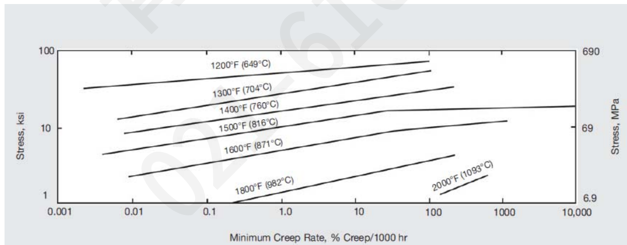
Figure 11 – Creep strength of solution-treated material.
