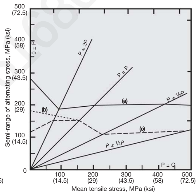
Figure 22. Fatigue test at 480°C (896°F)
