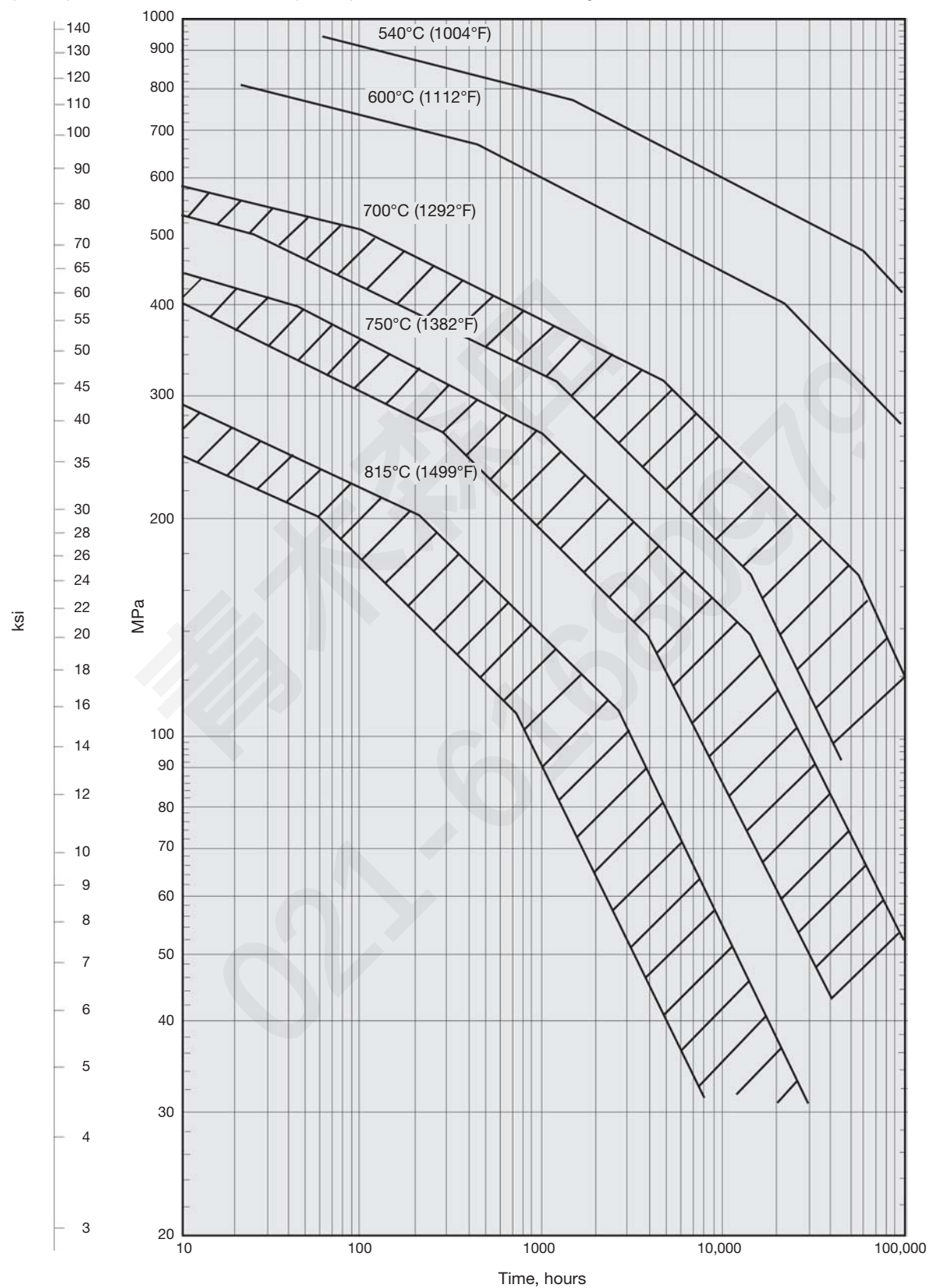
Figure 12 . Creep properties of NIMONIC alloy 80A extruded bar, subsequently forged. Heat treatment 8 hours/1080°C (1976°F)/air cooled + 16 hours/700°C (1292°F)/air cooled. 98% confidence region on 16-18 casts.
