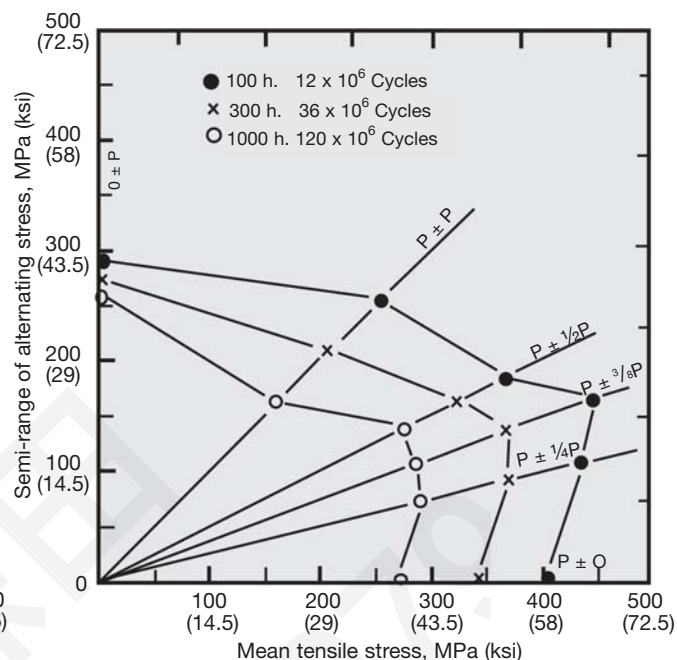
Figure 20. Fatigue test at 700°C (1292°F)
