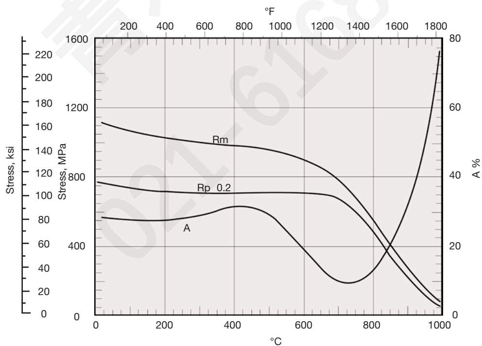
Figure 10. Tensile properties of rolled sheet. Heat treated 2 to 3 minutes/1150°C (2102°F)/fluidized bed quenched + 20 minutes/1040°C (1904°F)/air cooled + 4 hours/750°C (1382°F)/air cooled. Average results of tests on 5 casts.
