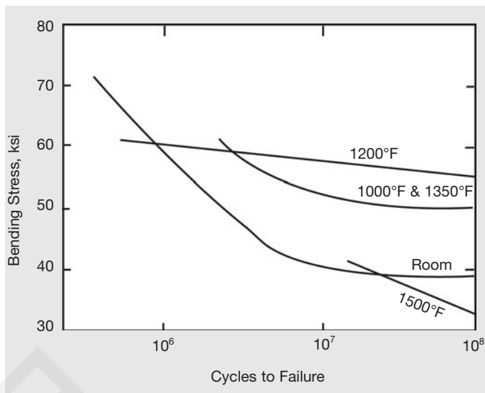
Figure 12. High-temperature fatigue strength of 5/8-in.-dia. hot-rolled bar triple-heat-treated (2100°F/2 hr + 1550°F/24 hr + 1300°F/20 hr). Samples tested in completely reversed bending.
