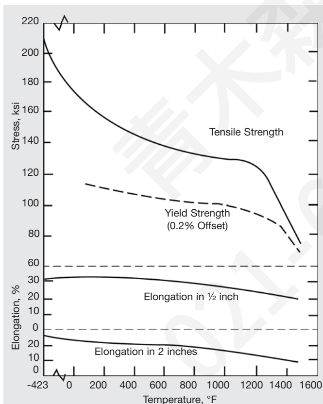
Figure 39. Tensile properties of welded 3/4-in. plate. Welded by gas tungsten-arc process. Double U-groove butt weld. Postweld heat treatment, 1925°F/1 hr, A.C.+1300°F/20 hr.
