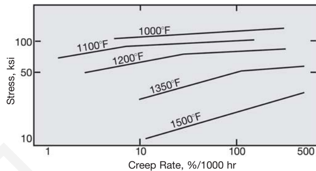
Figure 6. Creep properties of hot-rolled bar equalized and precipitation-treated (1625°F/24 hr, A.C., + 1300°F/20 hr, A.C.).
