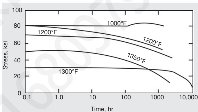
Figure 13. Relaxation of bar triple-heat-treated (2100°F/2 hr, A.C., + 1550°F/24 hr, A.C., + 1300°F/20 hr, A.C.).
