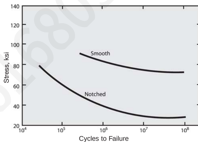
Figure 4. Fatigue strength of 3/4 -in. hot-rolled bar equalized and precipitation-treated ( 1625^{\circ}\text{F}/24\text{ hr, A.C.}, + 1300^{\circ}\text{F}/20\text{ hr, A.C.} ). R.R. Moore rotating-beam tests at 10,000 rpm. K_t=3.4 .
