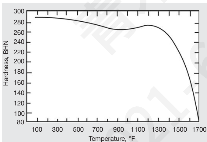
Figure 11. High-temperature hardness of hot-rolled material triple-heat-treated (2100°F/4 hr + 1550°F/24 hr + 1300°F/20 hr.).
