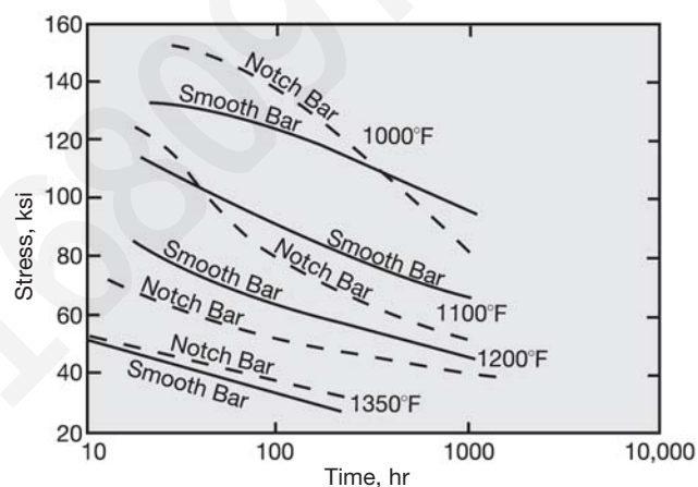
Figure 7. Rupture life of bar equalized and precipitation-treated (1625°F/24 hr, A.C., + 1300°F/20 hr, A.C.). Smooth bar, 0.3-in. dia. x 1 1/2 in. long; notched bar, 50% 60° V-notch, 0.005-in. root radius.
