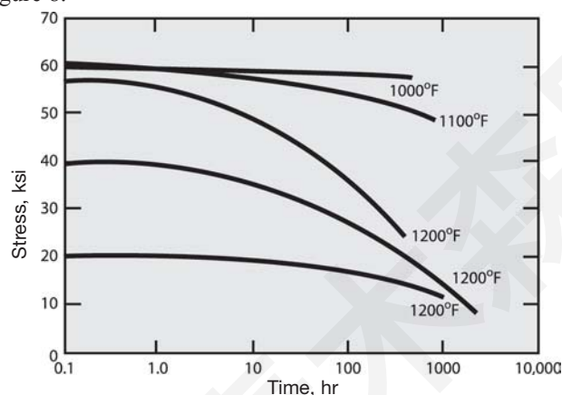
Figure 1. High-temperature relaxation of hot-rolled bar equalized and precipitation-treated ( 1625^{\circ}\text{F}/24\text{ hr, A.C.}, + 1300^{\circ}\text{F}/20\text{ hr, A.C.} )
