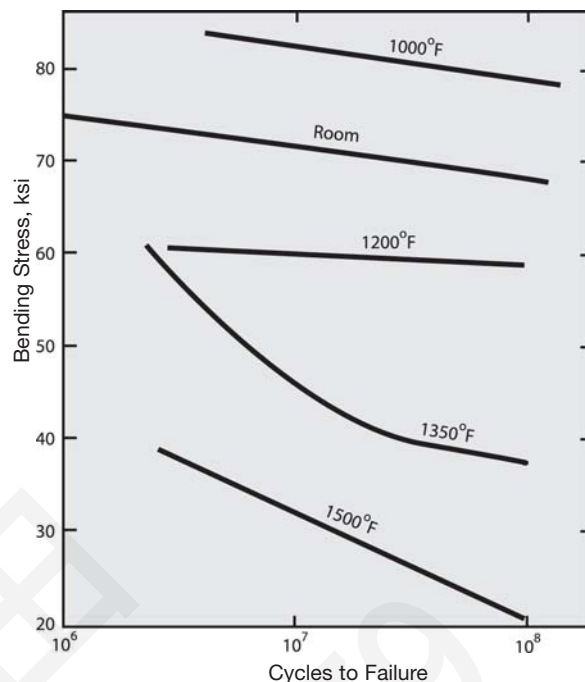
Figure 3. High-temperature fatigue strength of 5/8 -in.-dia. hot-rolled material equalized and precipitation-treated ( 1625^{\circ}\text{F}/24\text{ hr} + 1300^{\circ}\text{F}/20\text{ hr} ).
