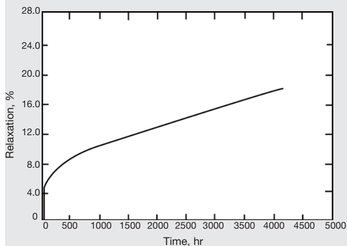
Figure 31 - Relaxation at 1300°F of Spring-Temper, triple-heat-treated springs. (Stresses corrected for curvature; modulus corrected for temperature.) Loaded at 20 ksi.
