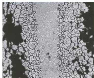
Alloy 800H Average Metal Affected = 23.2 Mils (590μm)/Side
