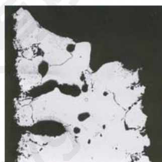
alloy 600 Average Metal Affected = > 22 Mils (560 μm)/Side
