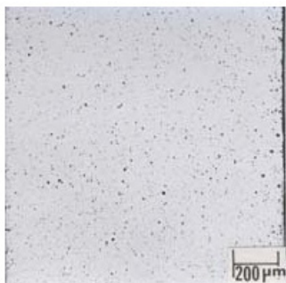
HAYNES® 556® alloy Average Metal Affected = 2.0 Mils (50 μm)/Side
