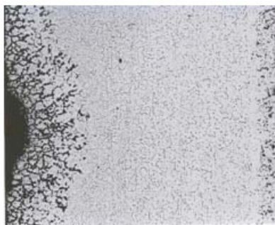
Type 310 Stainless Steel Average Metal Affected = 7.4 Mils (190μm)/Side
