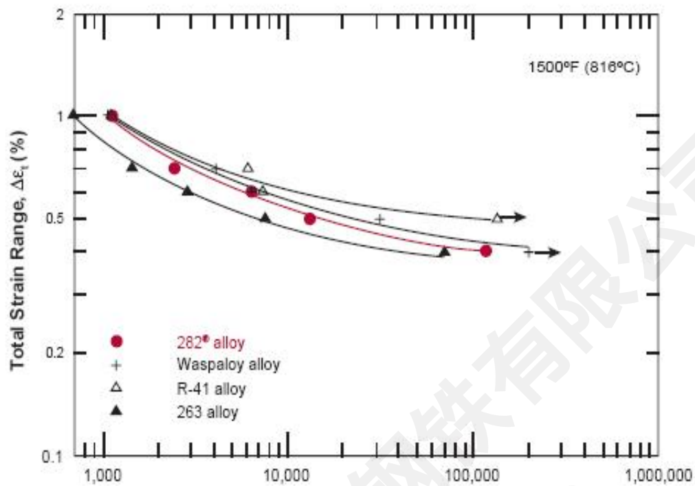
Comparative Low-Cycle Fatigue Data
