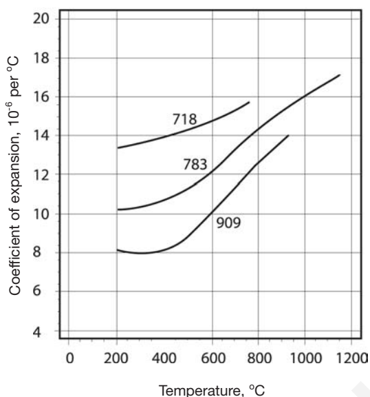
Figure 1- Mean coefficient of linear expansion between 25 ^{\circ}\text{C} and the temperature shown. (Alloys annealed and aged.)
