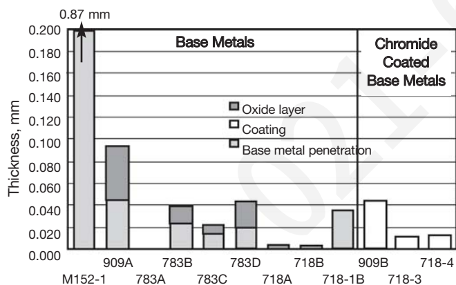
Figure 10 - Measurements of metal affected by 1,009 hours of salt spray at 35°C in 5% NaCl. Testing was done as per ASTM B117-97. Trends indicate the resistance alloy 783 is far superior to other low CTE alloys and on par with alloy 718. Letters and numbers after the alloy show multiple samples.
