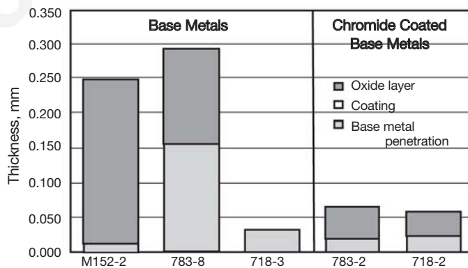
Figure 11 - Extent of corrosive attack after 1,009 hours of salt spray exposure and 649°C thermal exposure. Samples were tested as per ASTM B117-97 and also after intermittent exposure to 649°C for 24 hours twice a week.
