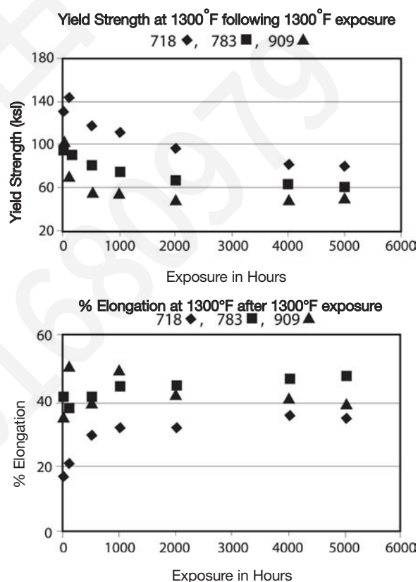
Figure 5 - High temperature tensile properties of INCONEL alloys 783, 718 and INCOLOY alloy 909 tested at 1300°F (704°C) following isothermal exposure at 1300°F (704°C).
