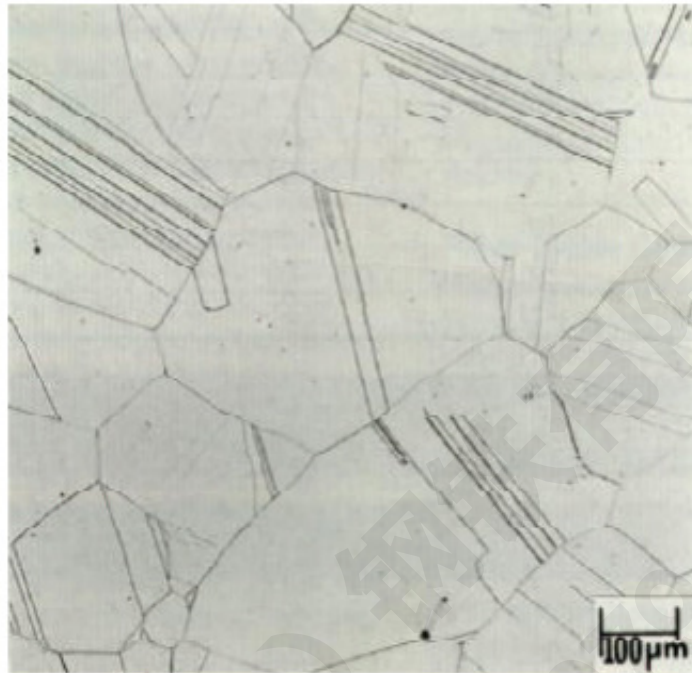
Annealed Microstructure
