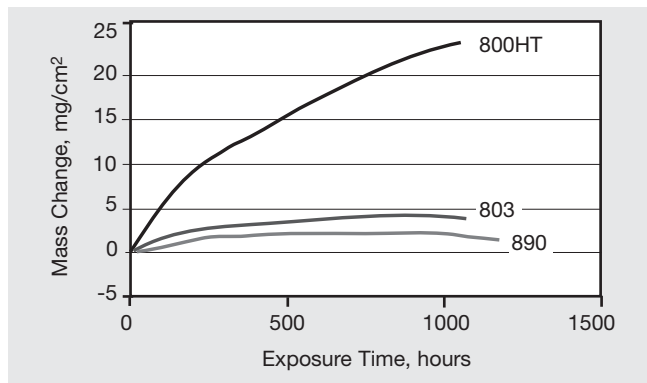
Figure 4. Mass change results after exposure in an oxidizing-carburizing atmosphere comprised of H_2 - 5.5% CH_4 - 4.5% CO_2 at 1000°C.
