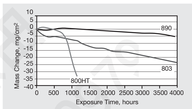
Figure 7. Mass change results after exposure in an air + 5% H_2O at 1000°C.
