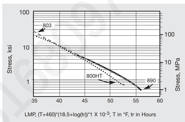
Figure 2. Larson-Miller plot showing relative creep rupture properties of as-produced INCOLOY alloys 803, 890 and 800H/HT.
