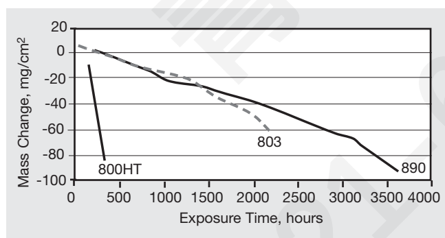
Figure 8. Mass change results after exposure in an air + 5% H_2O at 1100°C.
