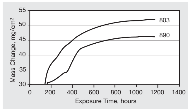
Figure 5. Mass change results after exposure in a carburizing atmosphere comprised of H_2 - 1% CH_4 at 1100°C.
