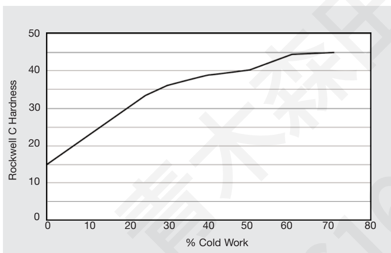
Figure 9. Work Hardening Curve for INCONEL alloy 693
