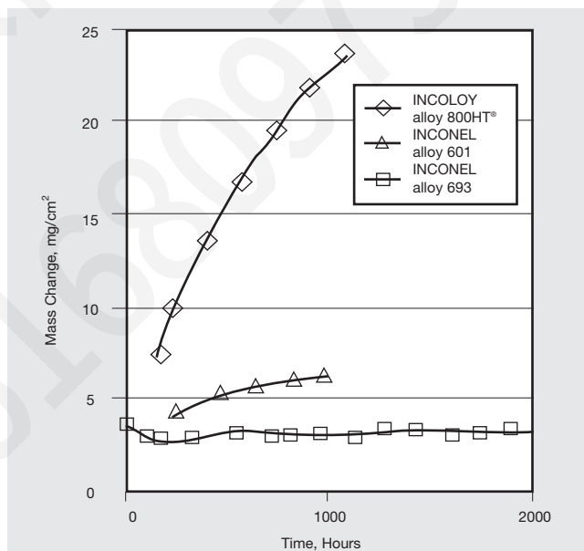
Figure 8. Mass change resulting from exposure in H 2 -5.5% CH 4 -4.5% CO 2 at 1000°C (1832°F).
