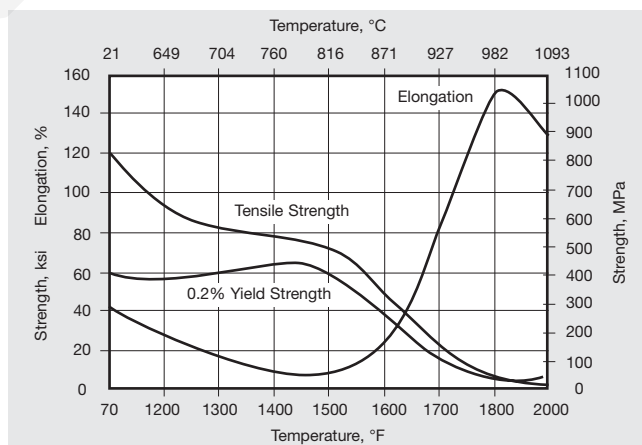
Figure 1. Elevated temperature tensile properties of annealed bar.
