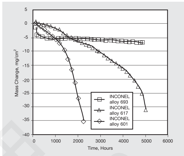
Figure 7. Oxidation resistance in air + 5% water at 1100°C (2012°F).
