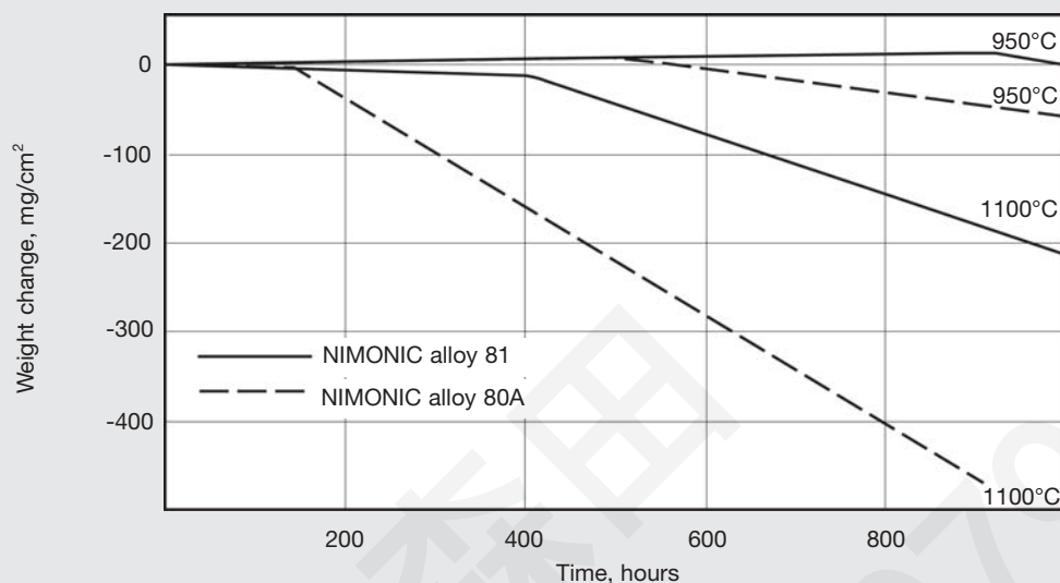
Figure 8. Cyclic oxidation properties of NIMONIC alloys 80A and 81 (Heating cycle: 20 minutes at temperature, 10 minutes at room temperature)
