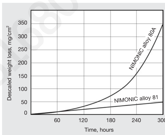
Figure 7. Intermittent salt shower corrosion tests (75% Na 2 SO 4 + 25% NaCl at 800°C)
