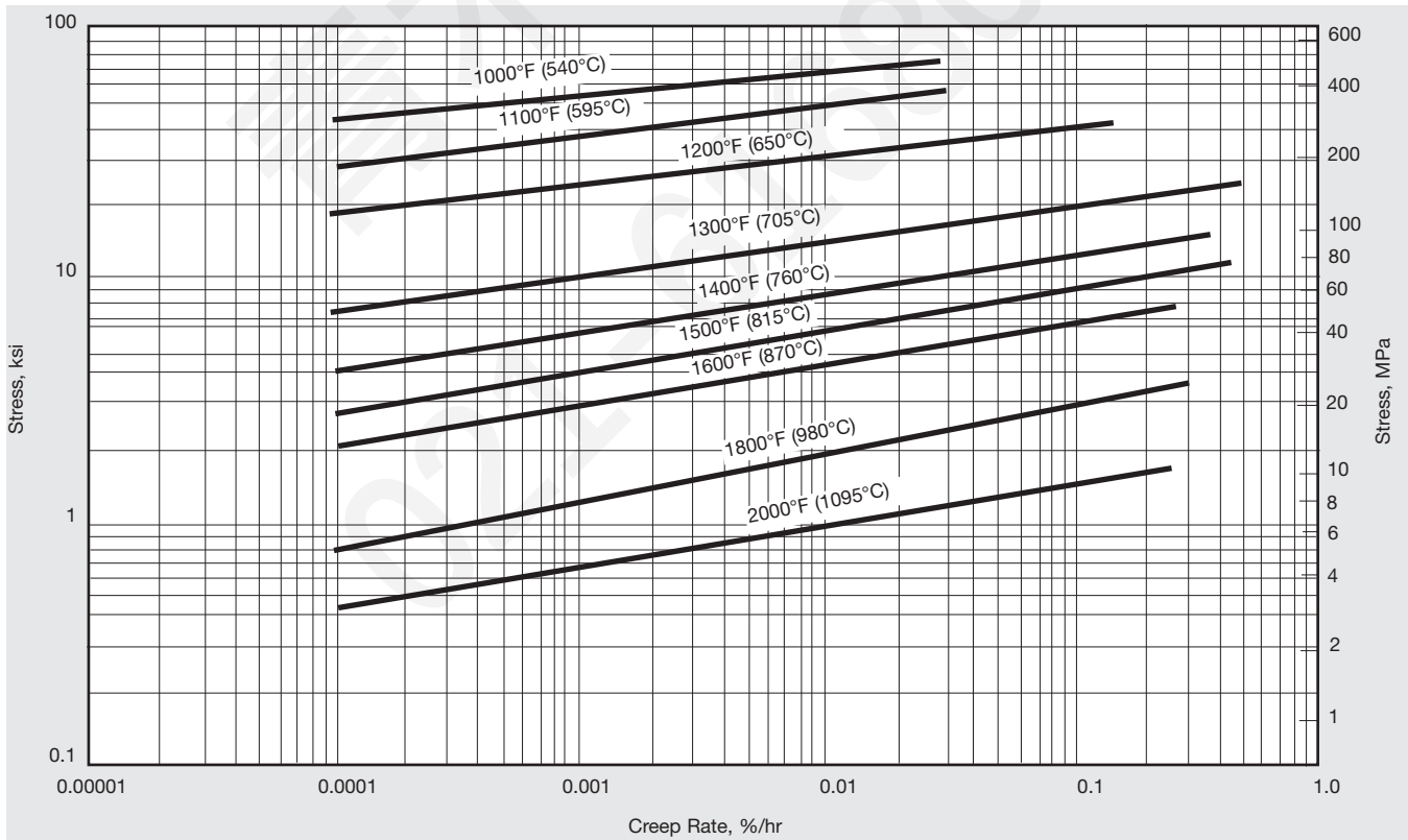
Figure 6. Typical creep strength of solution-treated (2100°F) (1150°C) INCONEL alloy 601.
