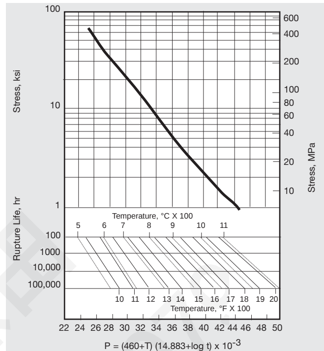
Figure 5. Larson-Miller parameter plot of rupture strength of solution-treated (2100°F) (1150°C) INCONEL alloy 601. In the parameter, T is temperature in °F, and t is time in hours.
