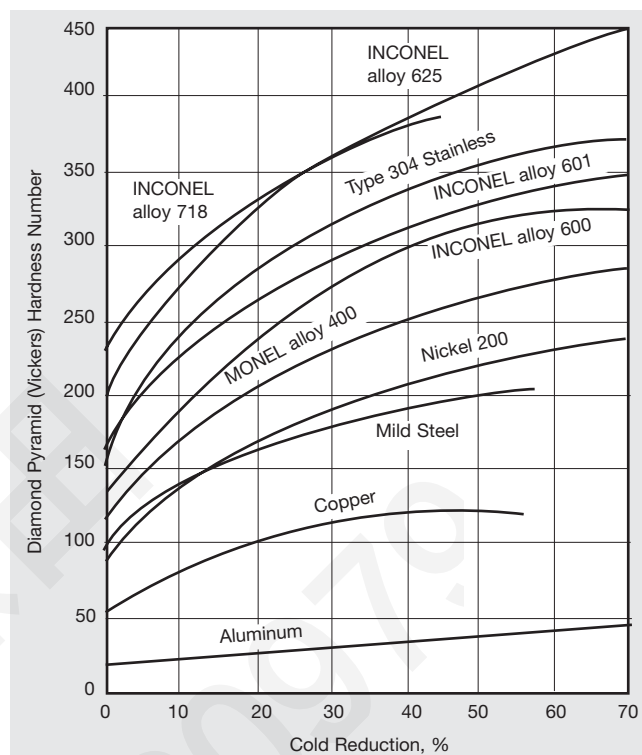
Figure 16. Work-hardening rates for INCONEL alloy 601 and other materials.
