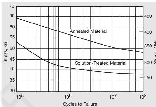
Figure 2. Rotating-beam fatigue strength at room temperature.
