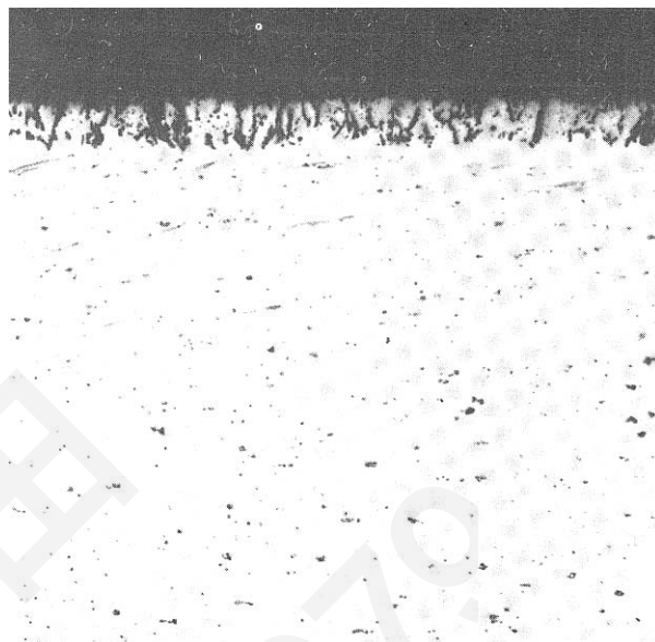
Figure 12. Oxide layer on specimen exposed to 2100°F (1150°C) for 500 hr. 75X. Unetched.
