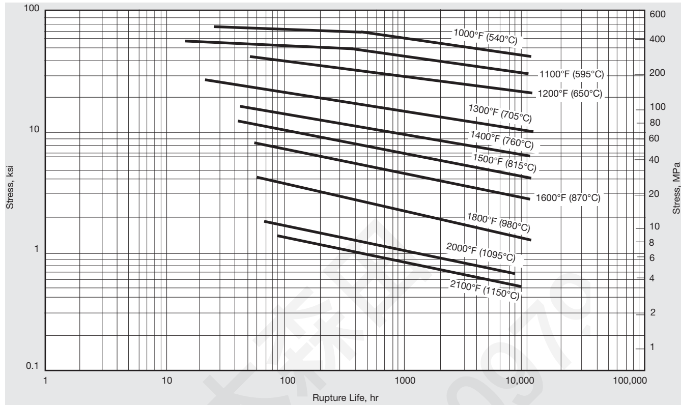
Figure 7. Typical rupture strength of solution-treated (2100°F) (1150°C) INCONEL alloy 601.
