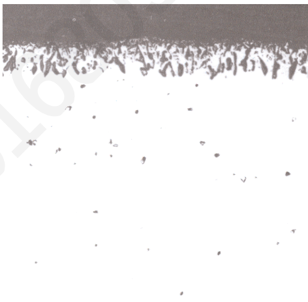
Figure 13. Oxide layer on specimen exposed to 2200°F (1205°C) for 500 hr. 75X. Unetched.
