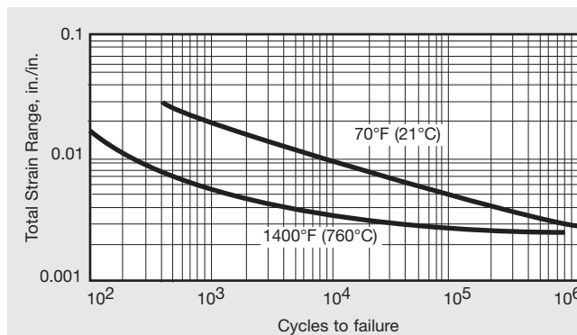
Figure 4. Low-cycle fatigue strength of INCONEL alloy 601.
